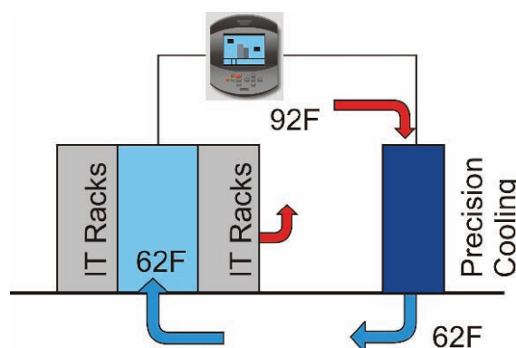
Figure 3.13: CAC with Intelligent Controller
