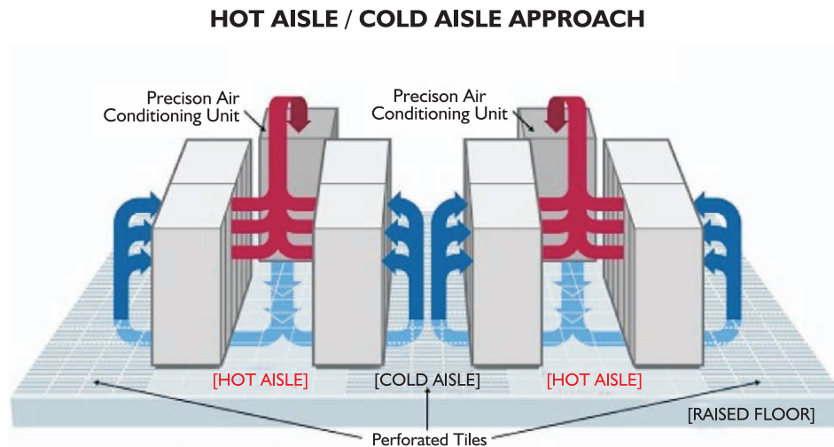
Figure 3.1: The raised floor of a Datacenter with the Hot aisle /Cold aisle setup
