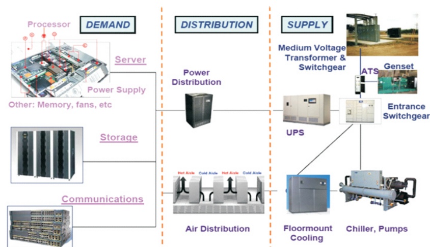
Figure 2: Typical Datacenter power consumption architecture
