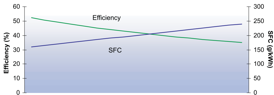
Figure 2.3: Illustration of SFC and efficiency relation
