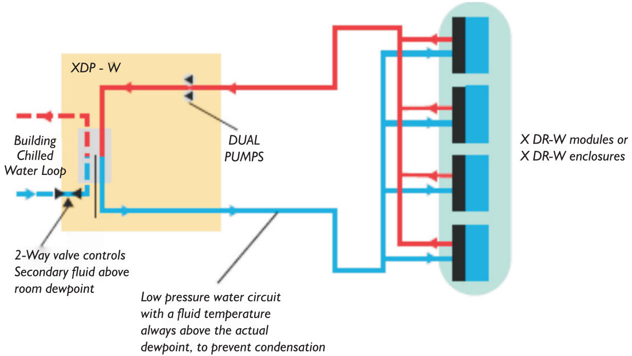
Figure 4.12b: Schematic of supplemental cooling
