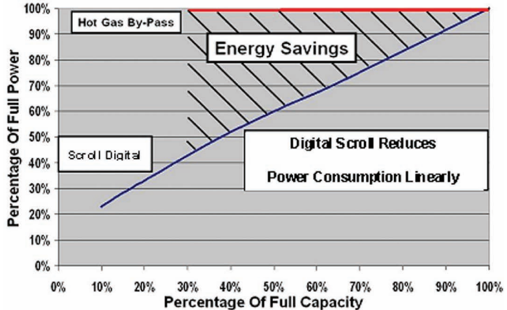
Figure 4.11: Percentage of full capacity (vs) Percentage of full power
