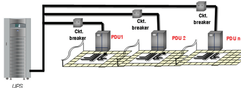
Figure 2.19: Diagram of Power Distribution from the UPS to the IT load through the PDU
