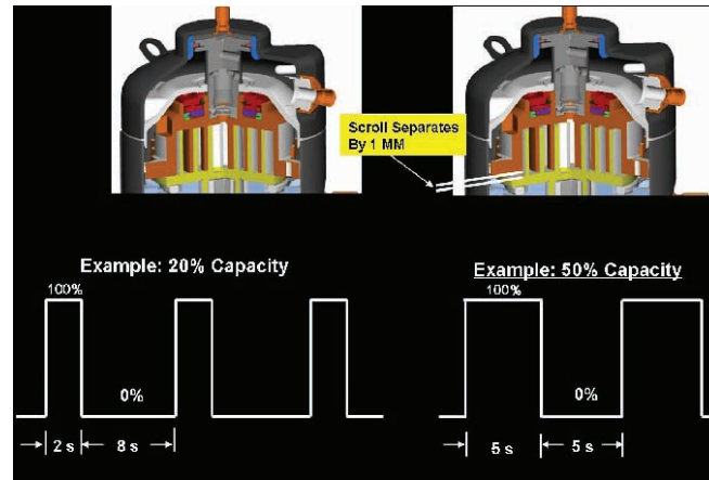
Figure 4.9: Scroll Compressors
