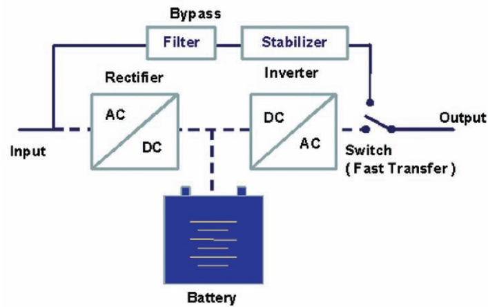
Figure 2.13: Line interactive UPS Configuration
