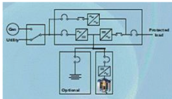
Figure 2.18 b: Schematic of a Flywheel based Static UPS
