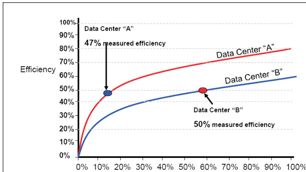
Figure 2.11: Comparison of the efficiency curves vs IT load for two different Datacenters
