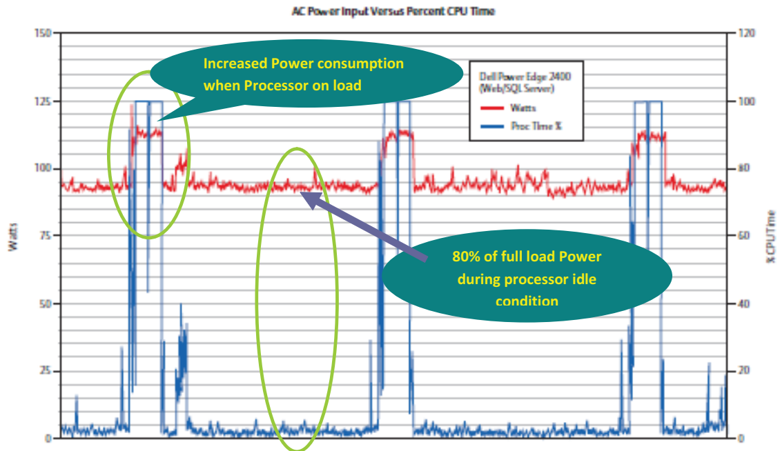
Figure 4.6: AC input power (vs) percent UPS time
