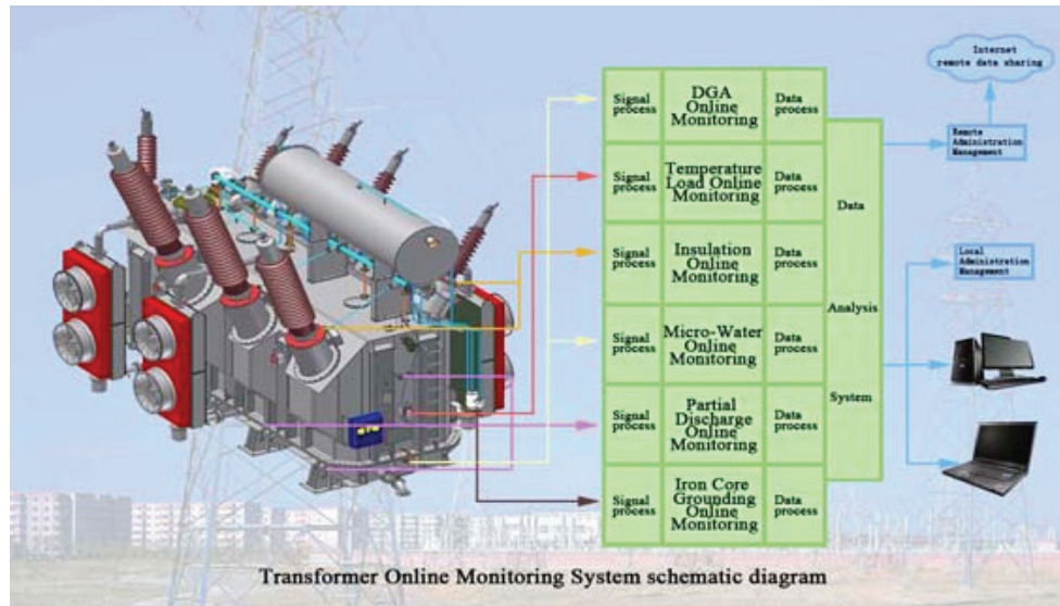
Figure- 5.2: Transformer online monitoring system
