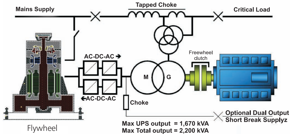
Figure 2.18 a: Schematic of Rotary UPS system
