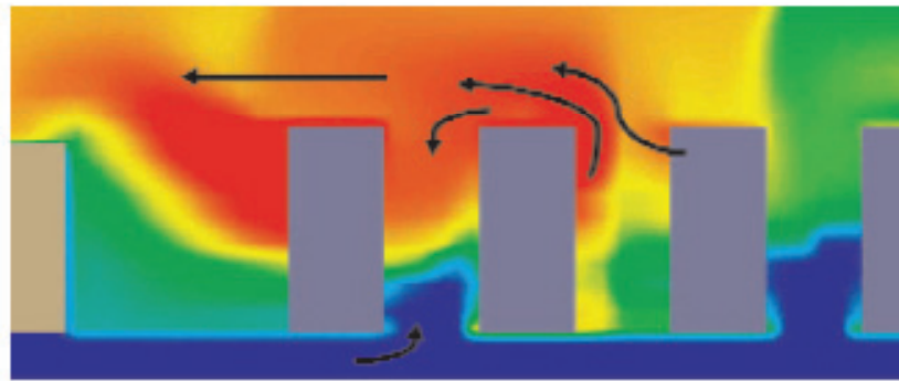
Figure 4.8: CFD Analysis
