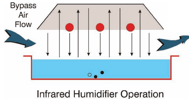
Figure 3.14: Infrared Humidifier Operation
