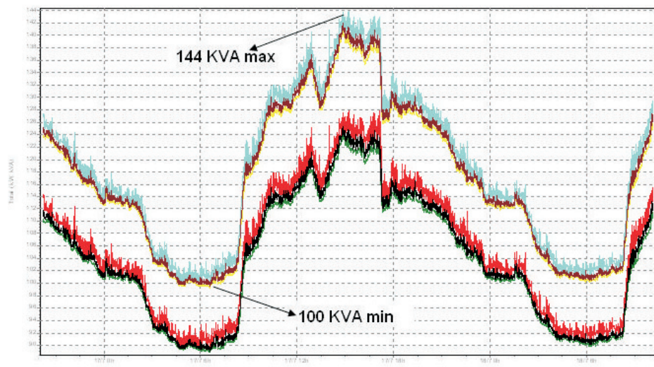
Figure 2.28: Loading pattern on UPS
