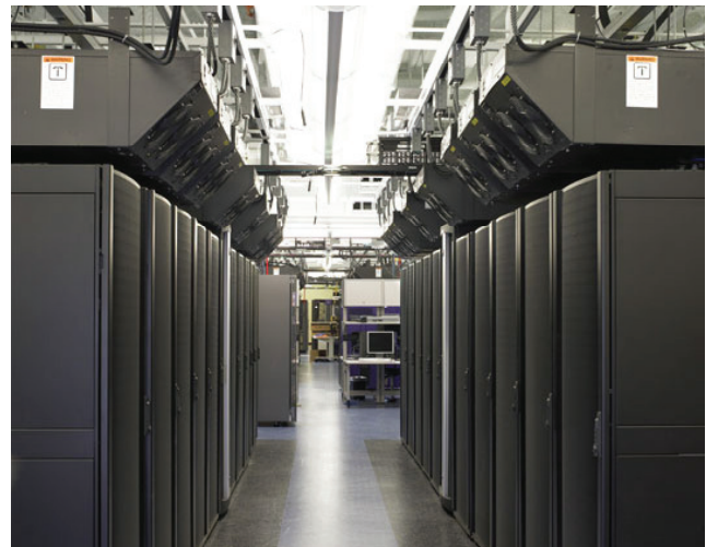
Figure 4.12a : Installation of high density supplemental cooling
