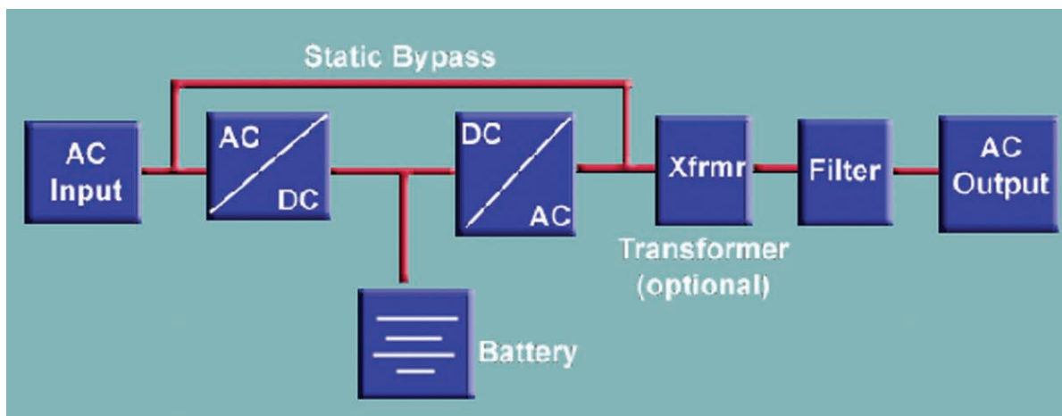
Figure 2.9: Typical Schematic diagram of Uninterruptible Power Supply
