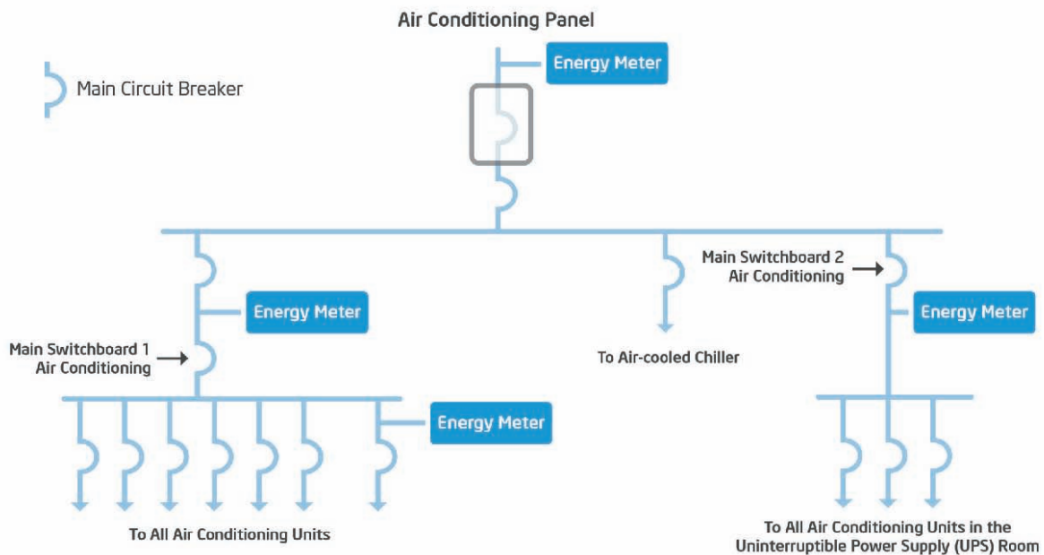
Figure 5.9: Cooling power metering isolated datacenter power from the facilities of the rest of the building
