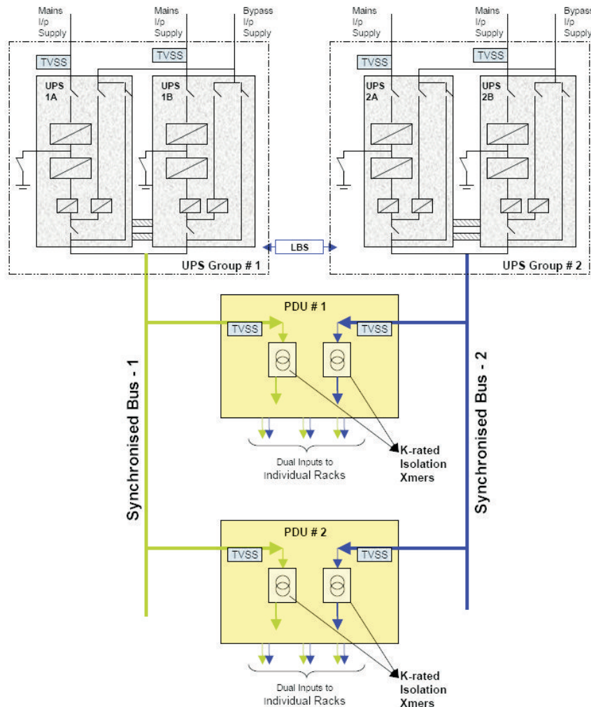
Figure 2.27: Schematic diagram of UPS configuration
