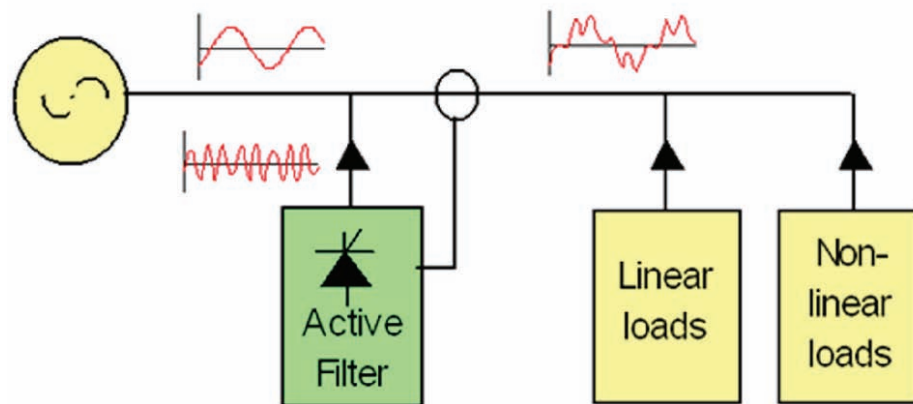
Figure 2.25: Typical Connection of an Active Harmonic Filter
