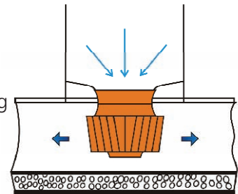
Figure 3.10a: Unique "In-Floor" Configuration
