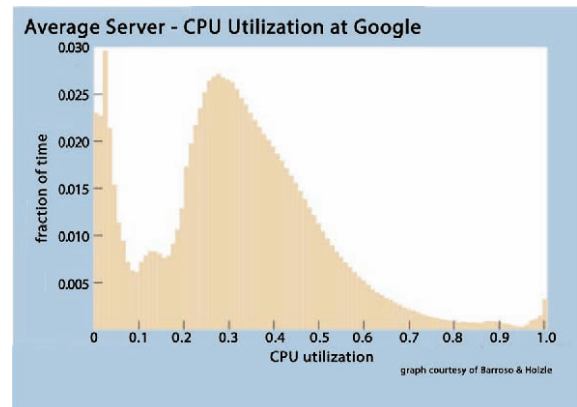
Figure 4.14: CPU utilization (vs) fraction of time
