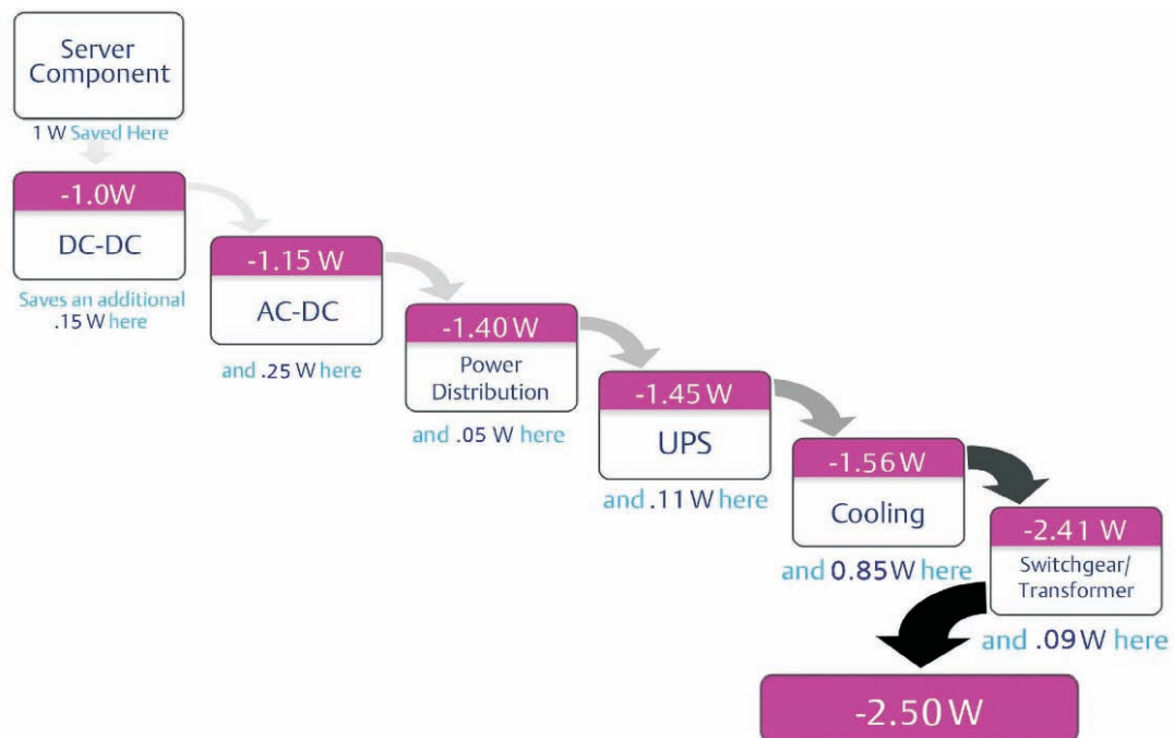
Figure 4.3: An estimated saving through “Cascading Effect”
