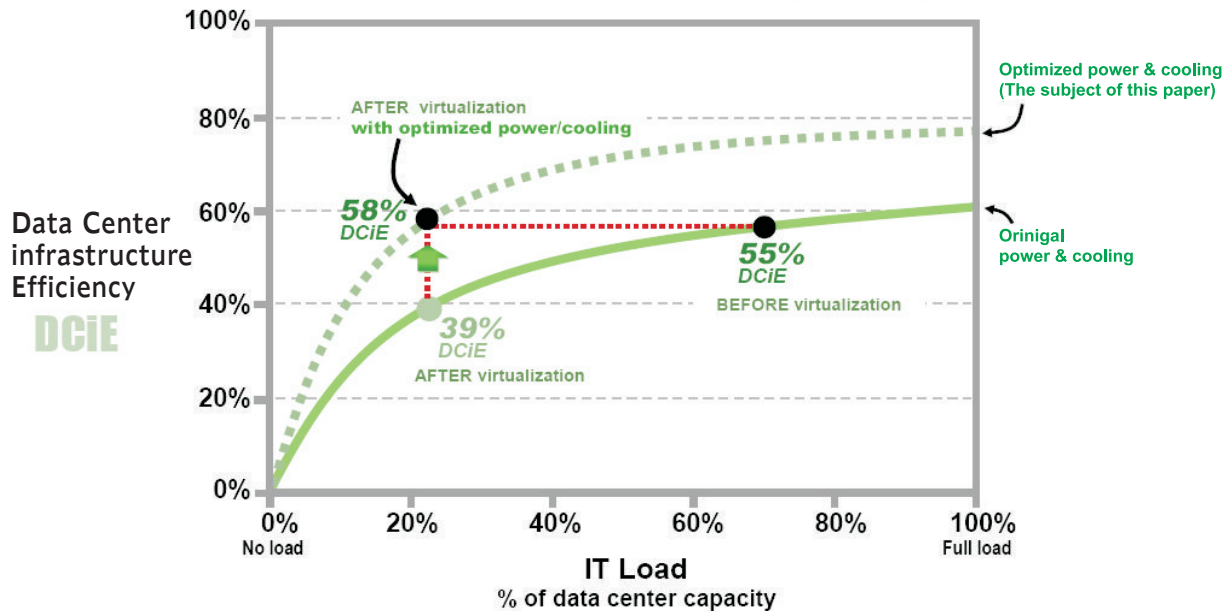
Figure 4.29 : Optimized Power and Cooling Raises the Efficiency Curve (Improves DCiE) (Source : APC)
