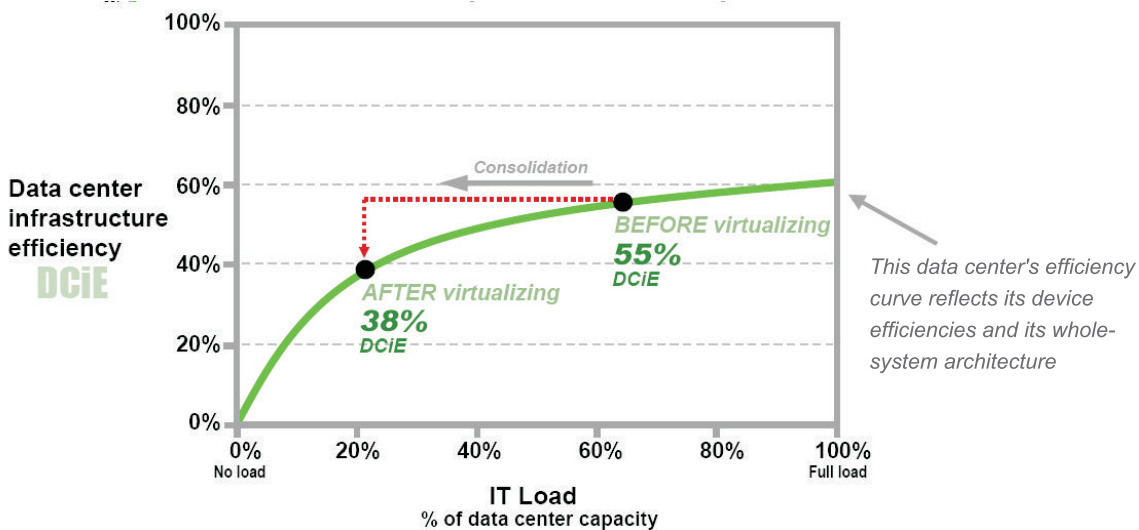
Figure 4.28 : Consolidation Reduces Infrastructure Efficiency if the Datacenter’s Infrastructure Remains Unchanged (Source : APC)
