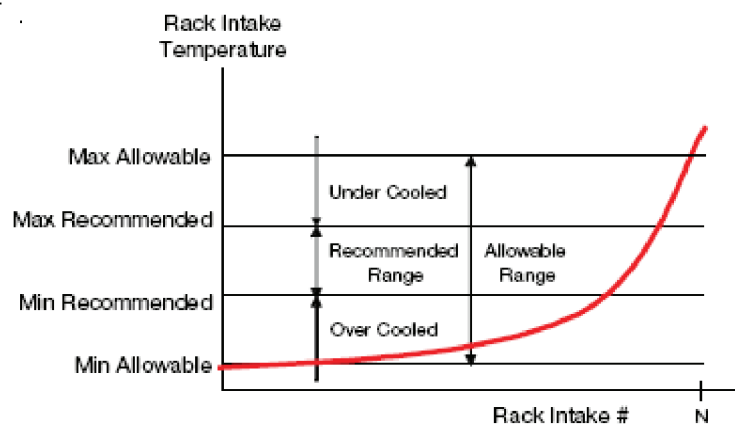
Figure – 5.6: Rack Intake (vs) Rack Intake temperature
