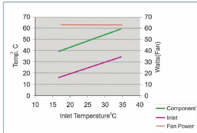
Figure 3.15: Inlet and Component Temperatures with fixed fan speed relative to increasing ambient temperature
