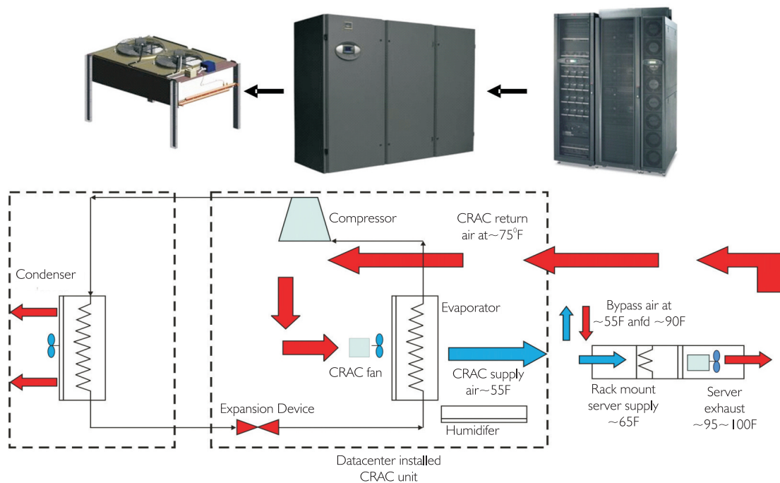
Figure 3.2: Typical Layout for direct expansion based precision cooling
