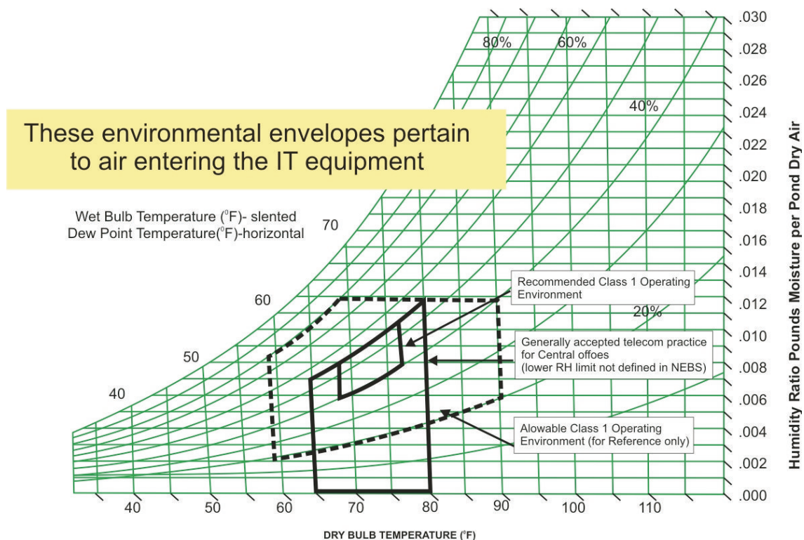
Figure 3.17: Dry Bulb temperature (vs) Humidity ratio
