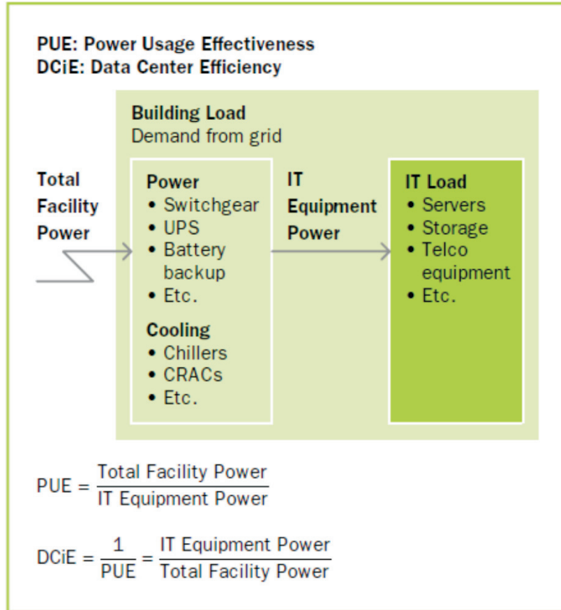
Figure - 5.5: Power flow in a Datacenter
