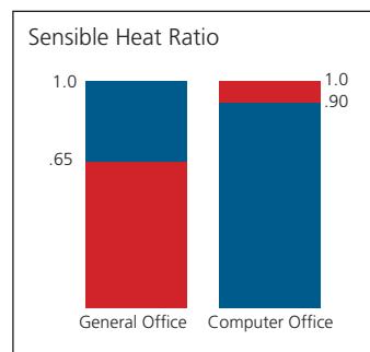
Figure 3.4a : Sensible Heat Ratio
