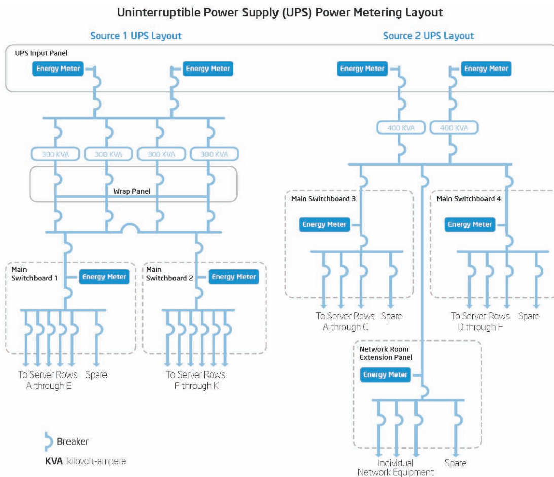
Figure 5.8: UPS metering layout to measure total IT power
