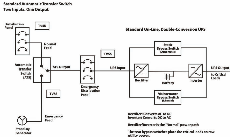
Figure 2.4: Schematic of Automatic Transfer switch Arrangement
