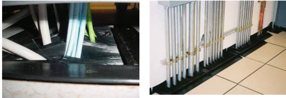
Figure 3.12 b : Installation of brush grommets
