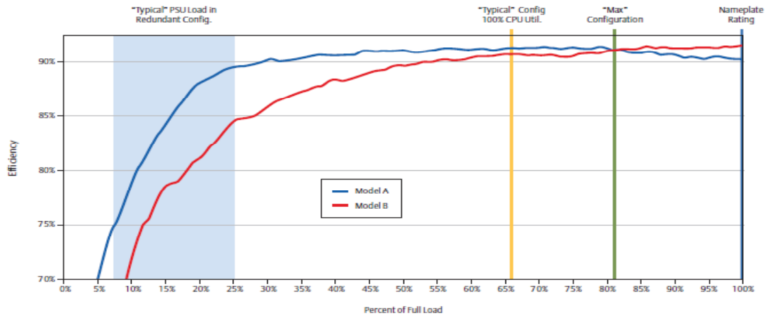
Figure 9. Power supply efficiency can vary significantly depending on load, and power supplies are often sized for a load that exceeds the maximum server configuration.
