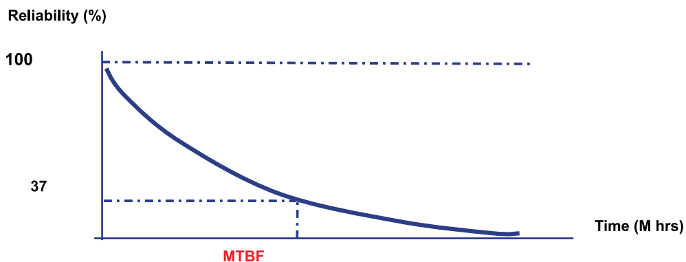
Figure 2.16: Graphical Representation of MTBF
