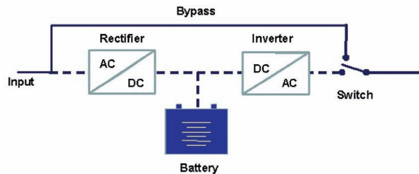
Figure 2.12: Block Diagram of Off Line UPS System
