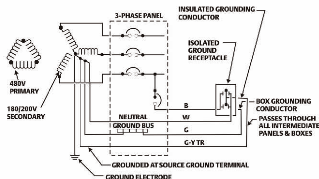
Schematic of Insulated Grounding
