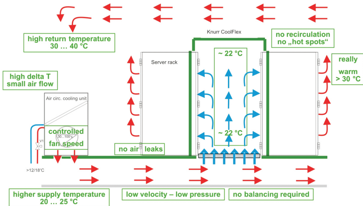
Figure 3.20: Typical arrangement of cold aisle containment
