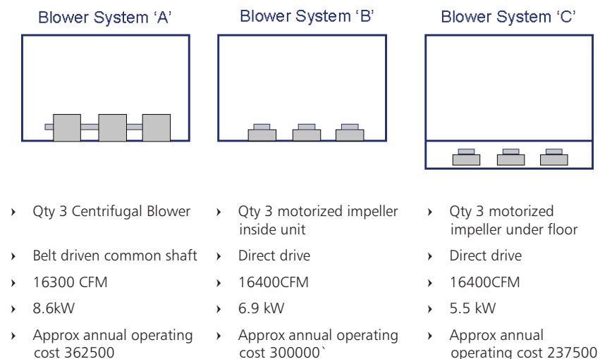
Figure 3.10 b: EC Fan configuration details
