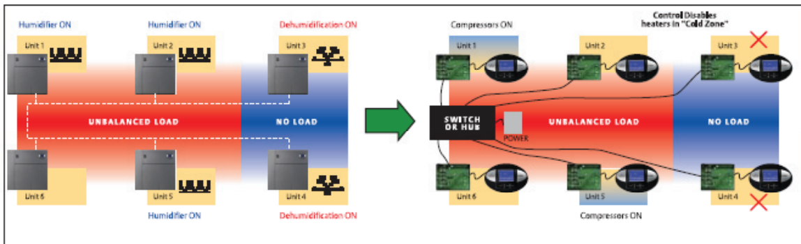
Figure 4.13: Schematic of CRAC unit with intelligent controller
