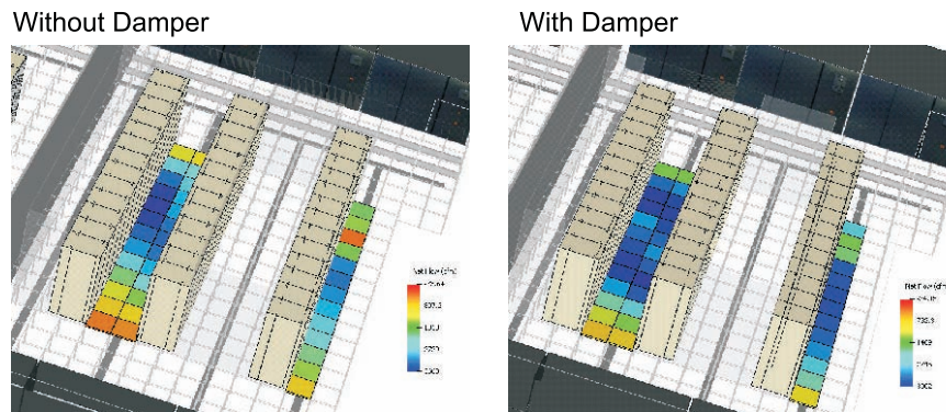
Figure 3.22: Floor Grill analysis
