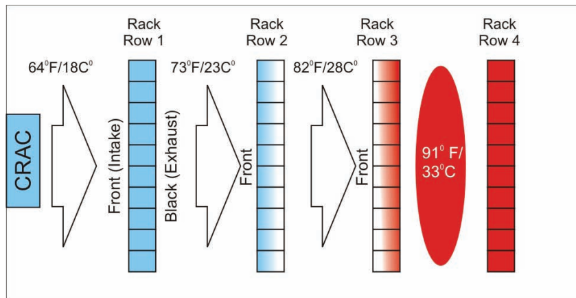
Figure 3.12a: Temperature difference of air to the server racks
