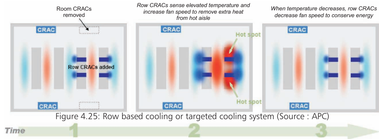
Figure 4.25: Row based cooling or targeted cooling system (Source : APC)
