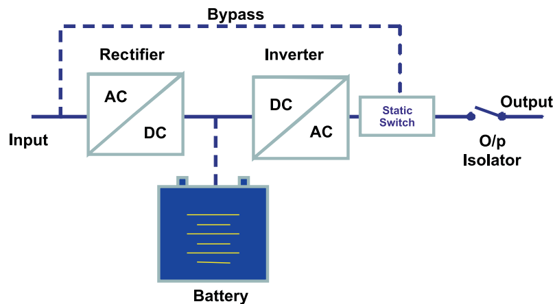
Figure 2.14: On-Line Double Conversion UPS Configuration
