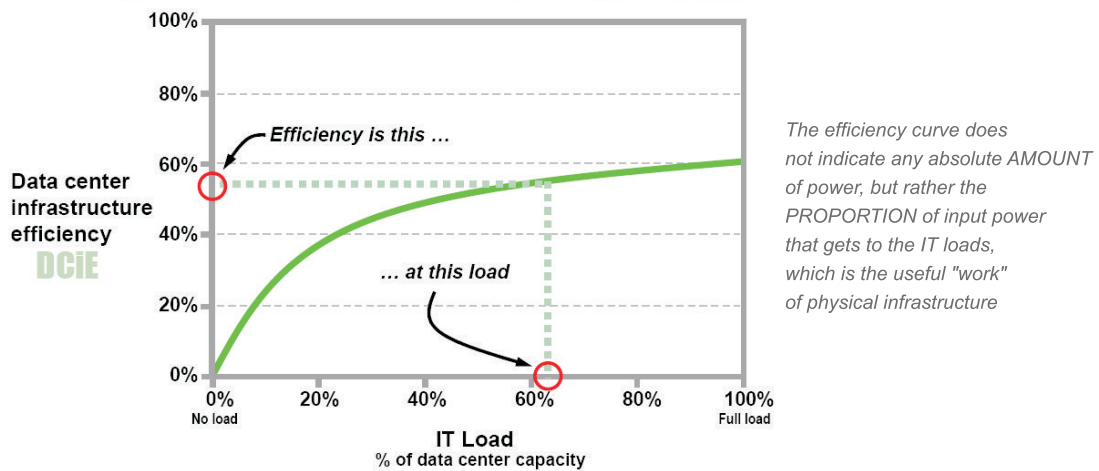
Figure 4.27 : Typical Datacenter Infrastructure Efficiency Curve (Source : APC)
