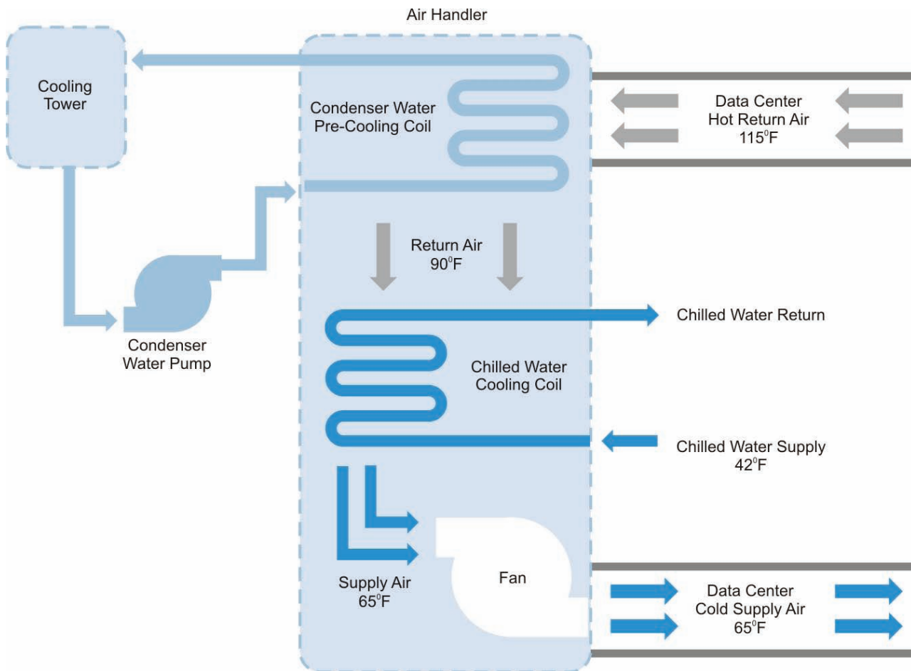
Figure 3.7: Schematic of Fluid based economizer
