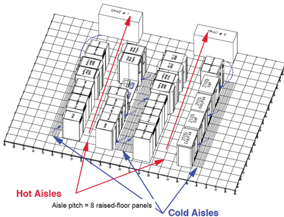
Figure 3.5: A typical layout of hot aisle and cold aisle approach
