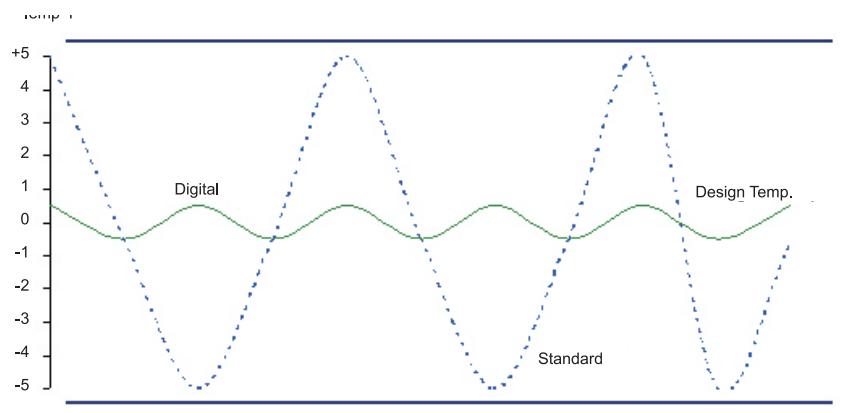
Figure 4.10: Temperature variation using Standard and digital scroll compressor
