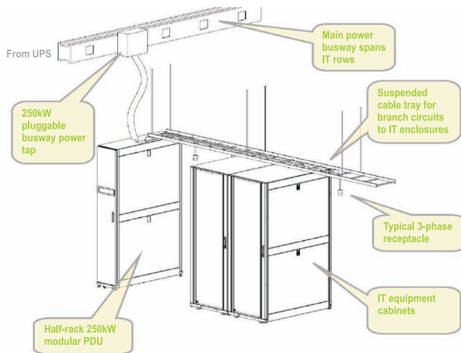
Figure 2.20: Schematic of Modular Power Distribution System [Source: APC]
