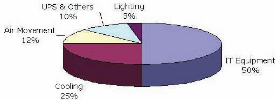
Figure 1: Power Usage Distribution in a Datacenter [Source: EYP Mission Critical Facilities Inc. New York]
