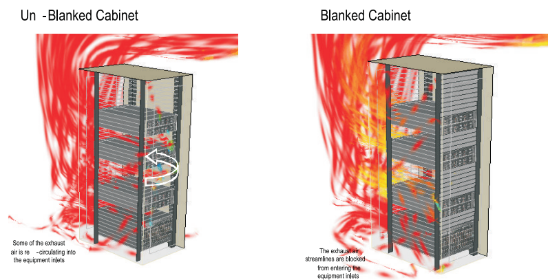
Figure 3.23: Rack analysis
