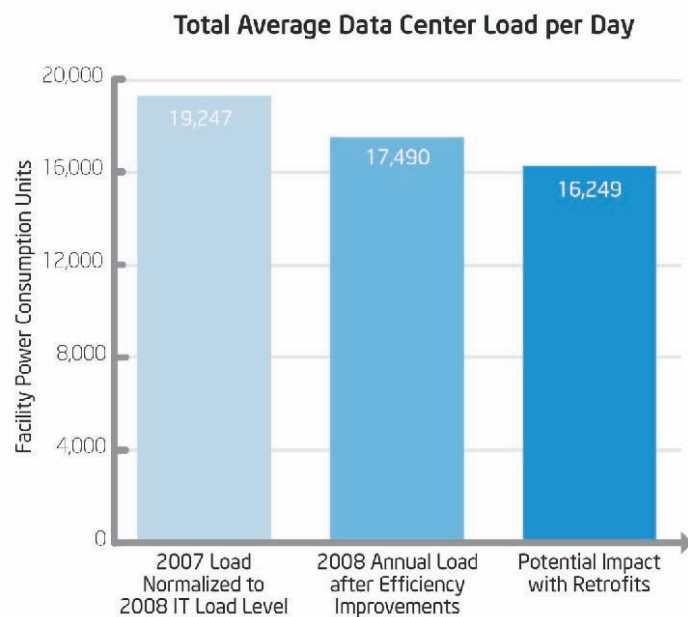
Figure 5.10: Total facilities load reduction
