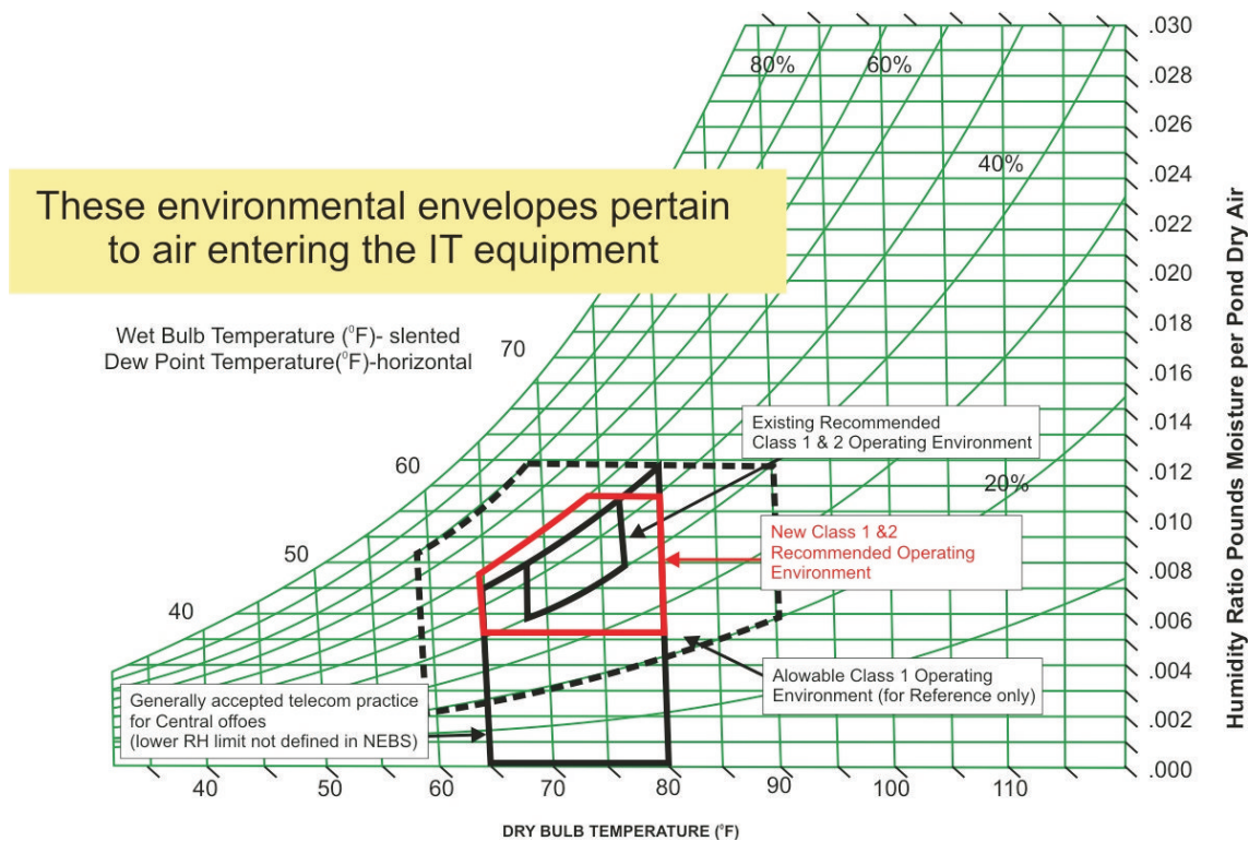
Figure 3.18: Recommended environment envelope data
