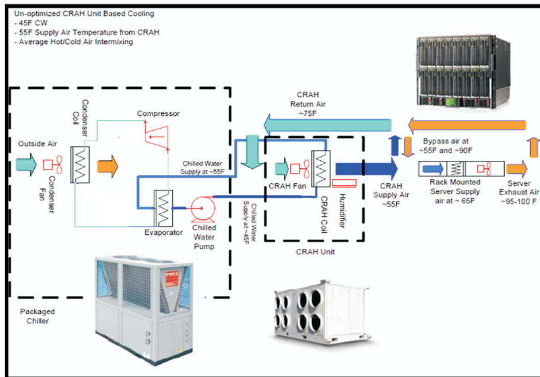
Figure 3.3: Typical layout for chilled water based precision cooling
