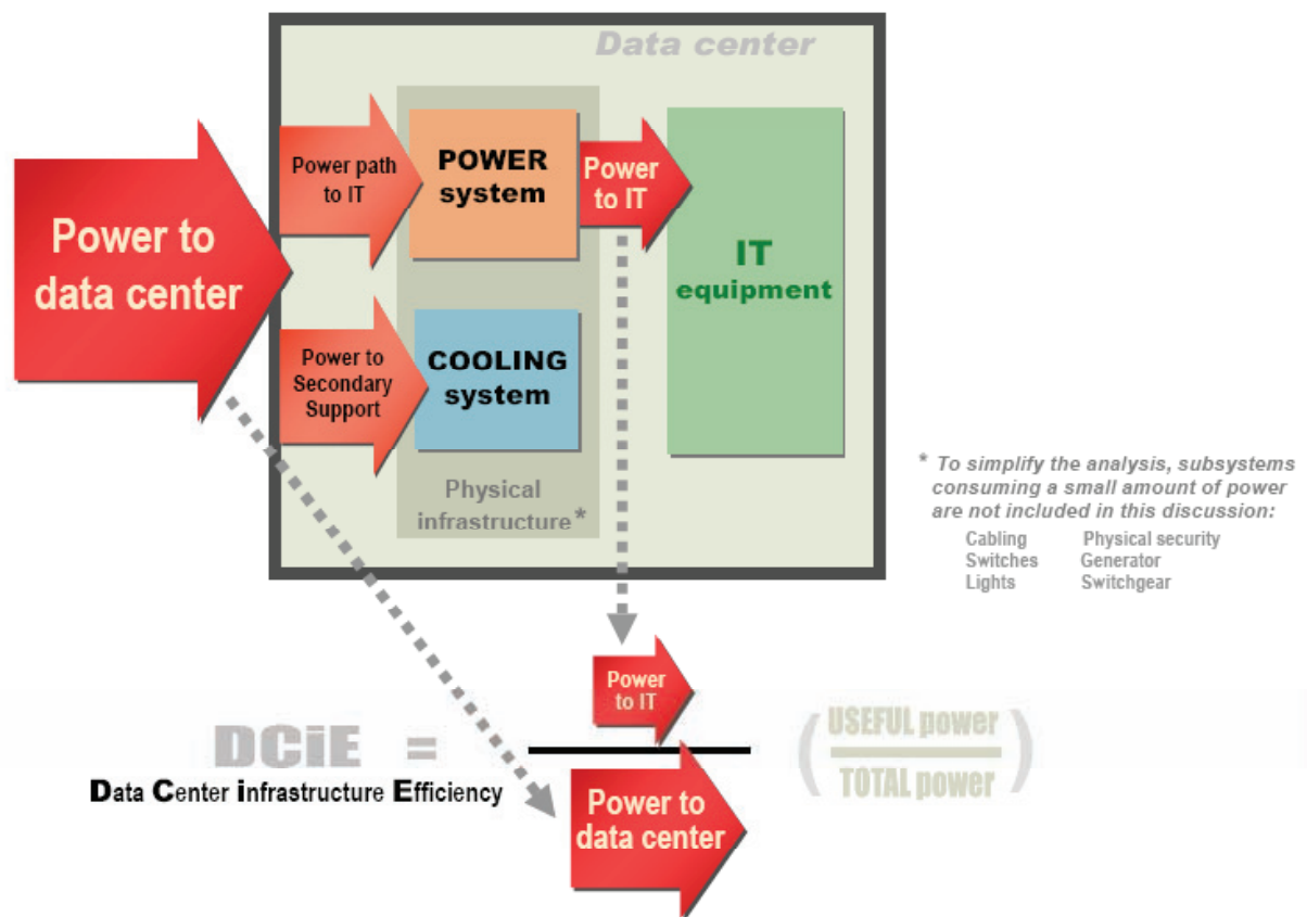
Figure 4.23 : Datacenter Infrastructure Efficiency (Source : APC)
