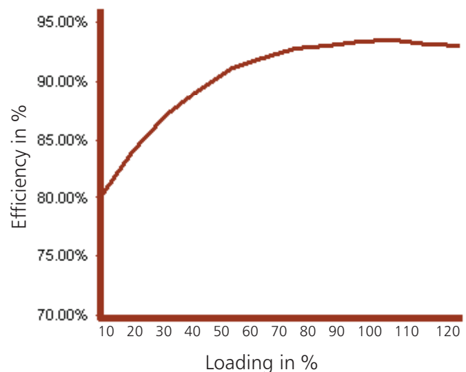
Figure 2.26: Loading (vs.) Efficiency curve of the UPS
