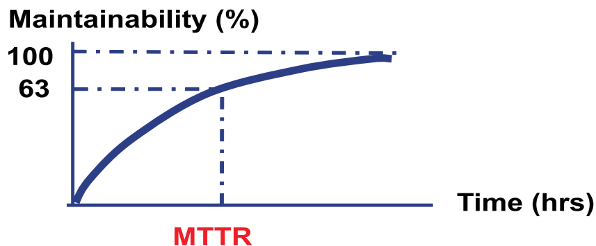
Figure 2.17: Graphical Representation of MTTR
