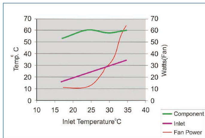
Figure 3.16: Inlet and Component Temperatures with variable fan speed relative to increasing ambient temperature
