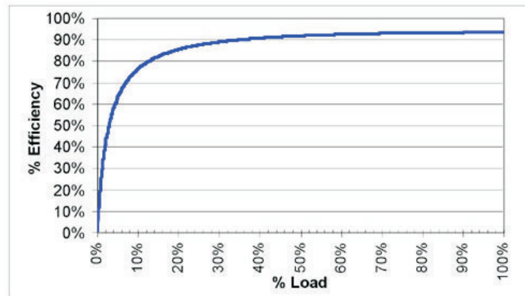
Figure 2.10: Loading versus. Efficiency Curve for a UPS
