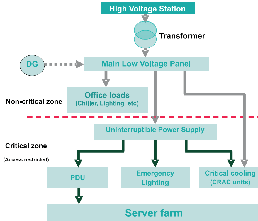
Figure 2.1: Power flow in a Datacenter
