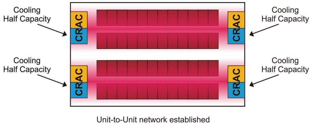
Figure 3.9 a: Capacity utilization in Team mode operation
