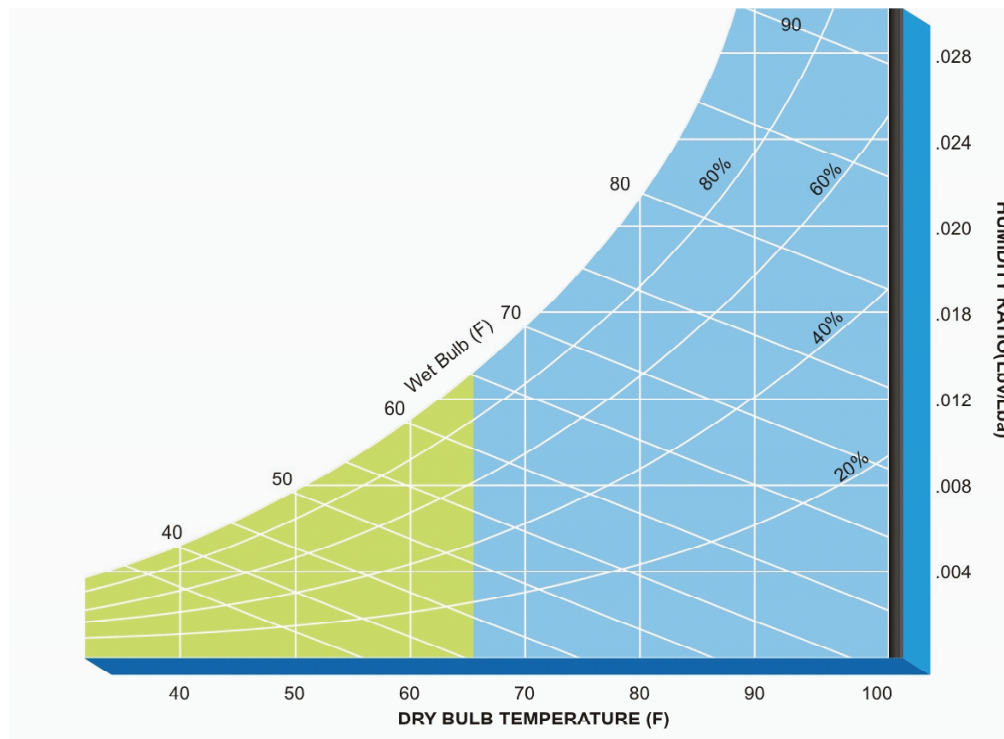
Figure 3.8: free cooling circuit (waterside economizer) operating range –Computer application
