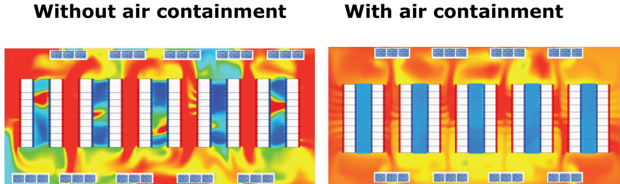
Figure 3.13b: CFD Analysis
