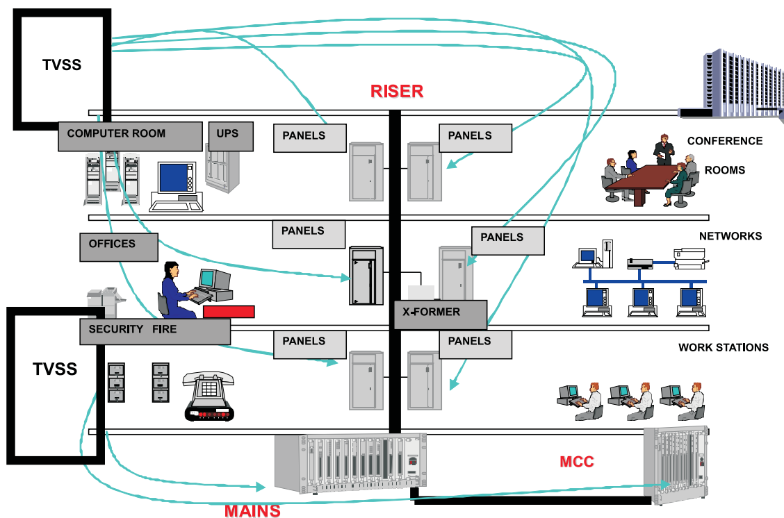
Figure 2.7: TVSS For Multistory Building shows the possibilities where TVSS is required
